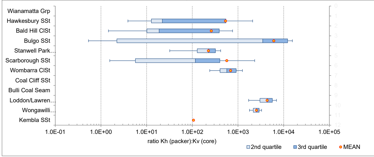
Figure 3-29 Summary of Hydraulic Conductivity data from core testing
