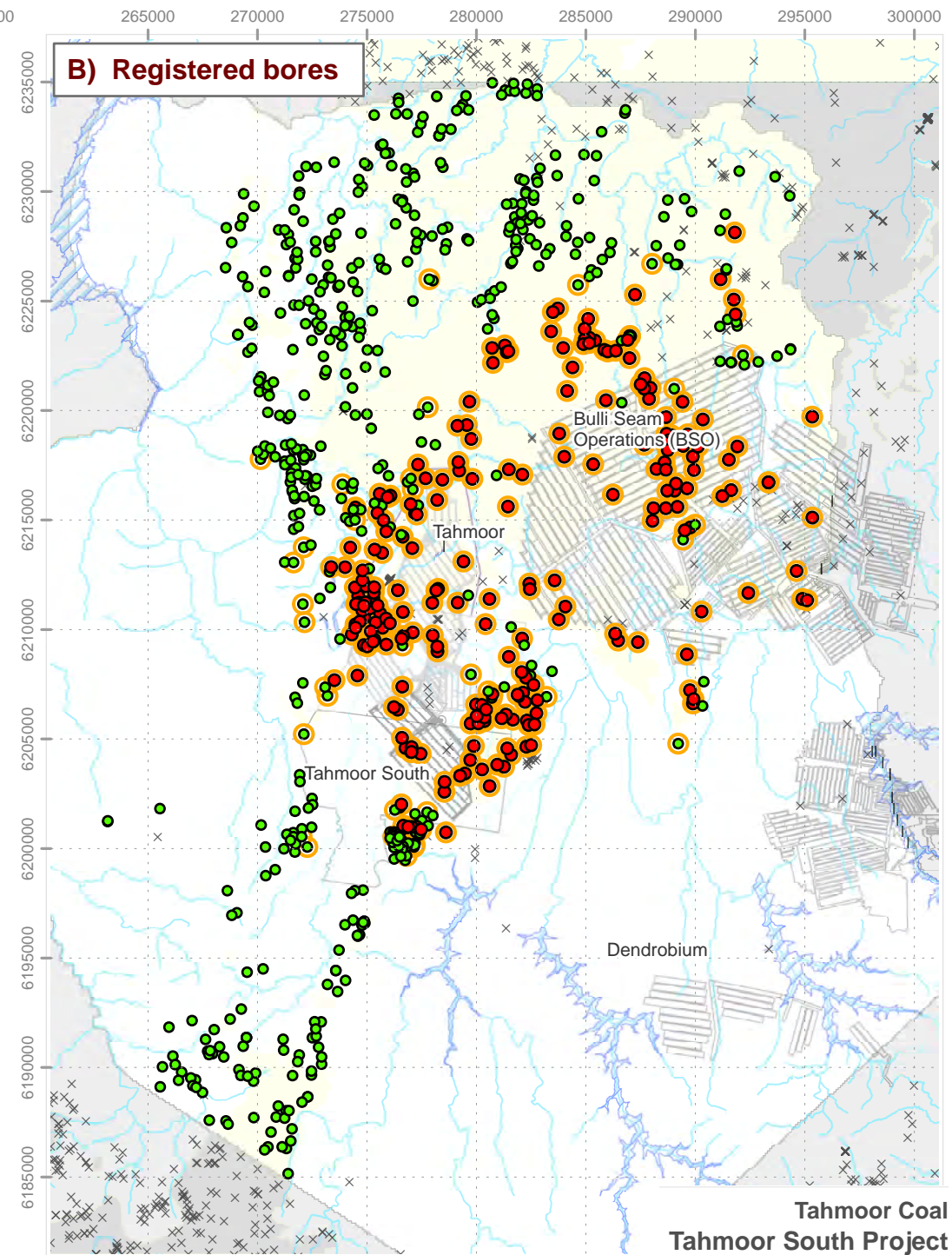
Effects at groundwater users: drawdown due to cumulative mining effects
