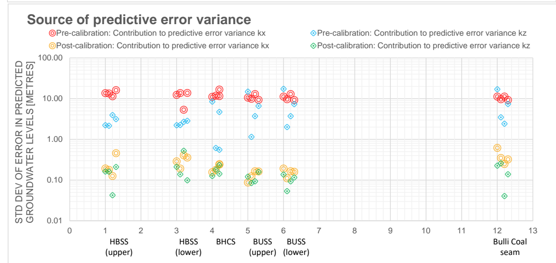
Figure 4-17 Summary of Uncertainty Analysis of Modelled Groundwater Levels
