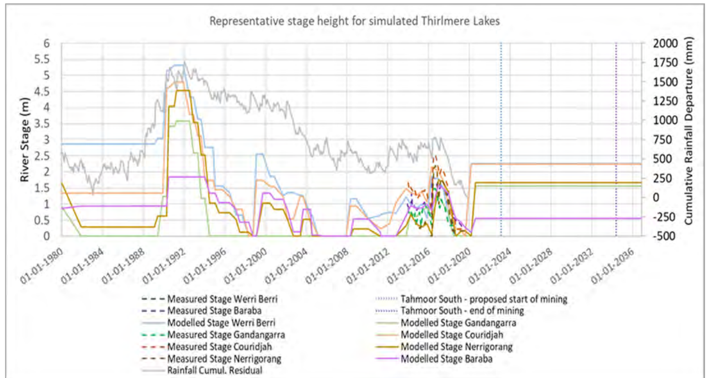
Figure 4-5 Modelled river stages applied to watercourses and Thirlmere Lakes
