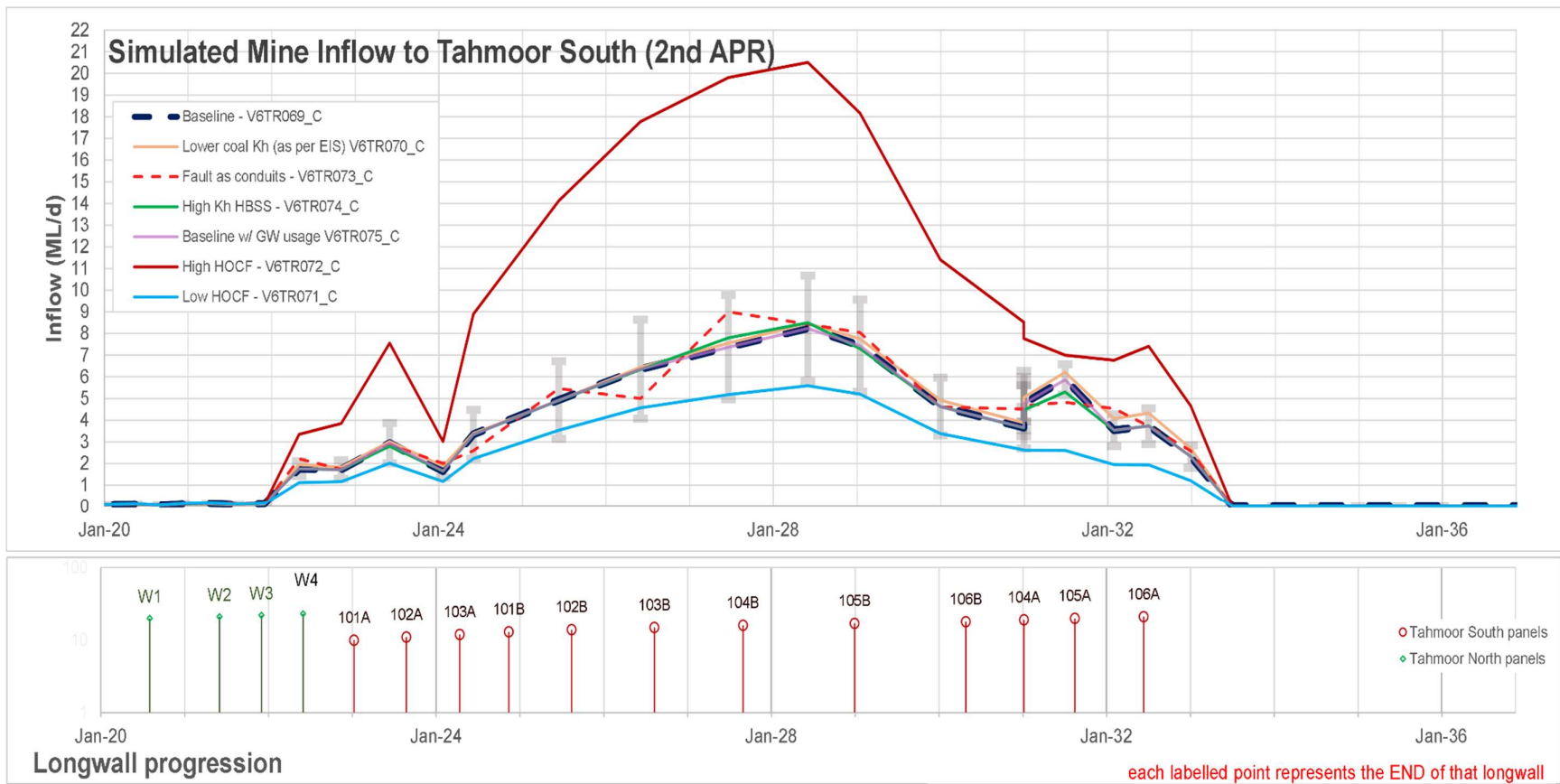
Figure 2 Predicted groundwater inflow (Second Amended Project)
