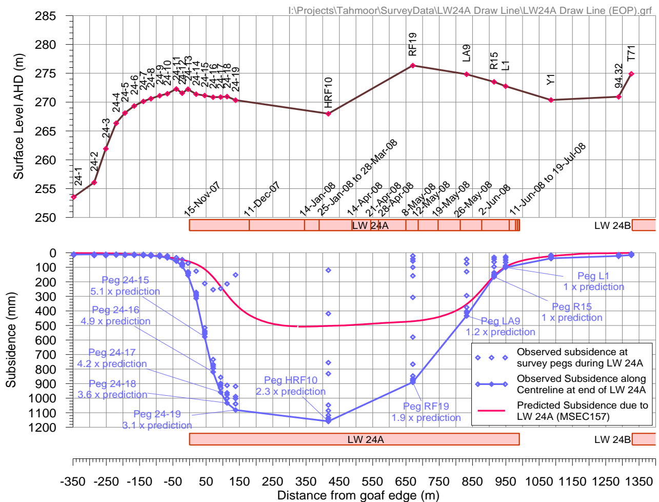
Figure. 2.1 Observed Subsidence along Centreline of Longwall 24A
