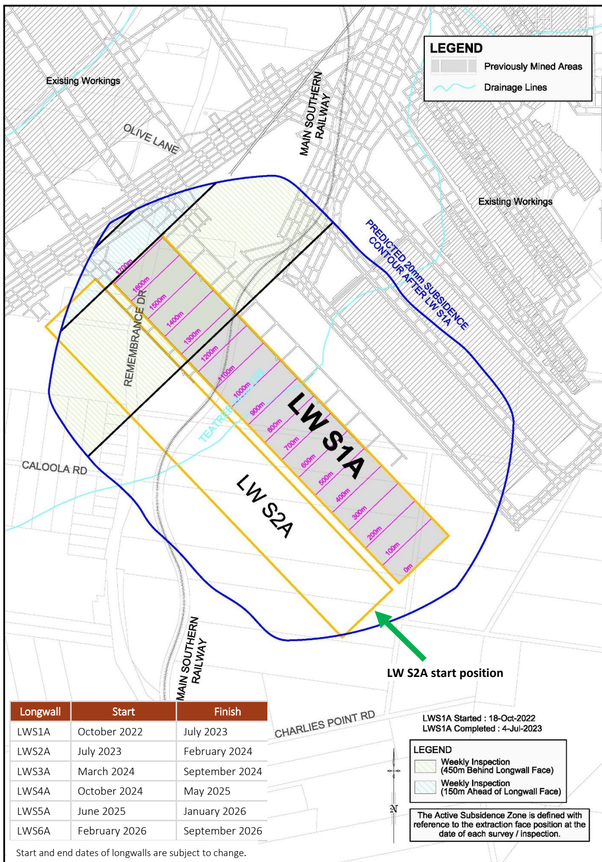
Figure 1 – Longwall South 1A subsidence zone
