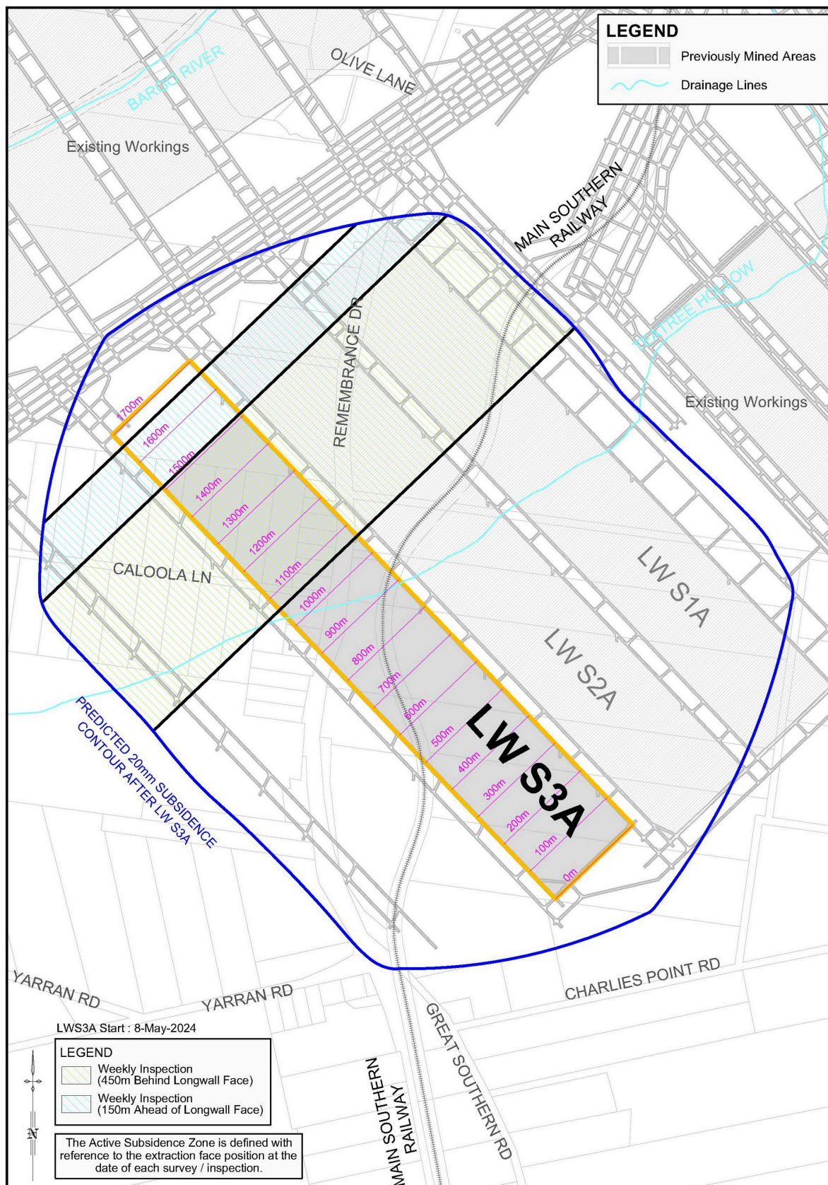
Figure 1 - Longwall South 3A subsidence zone
